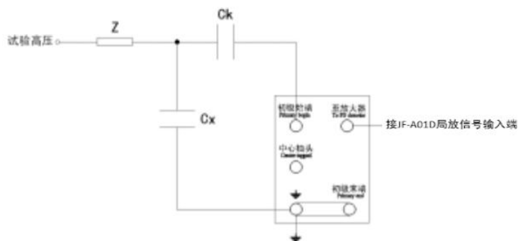
Figure 3a Parallel connection
