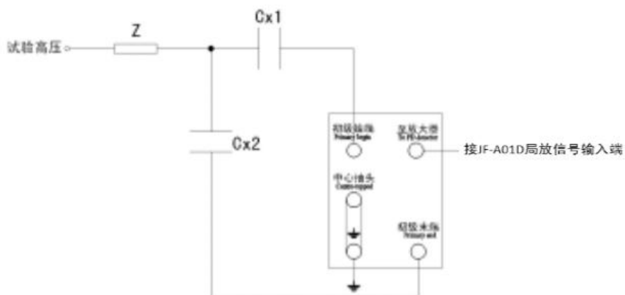
Figure 3c Balanced connection
