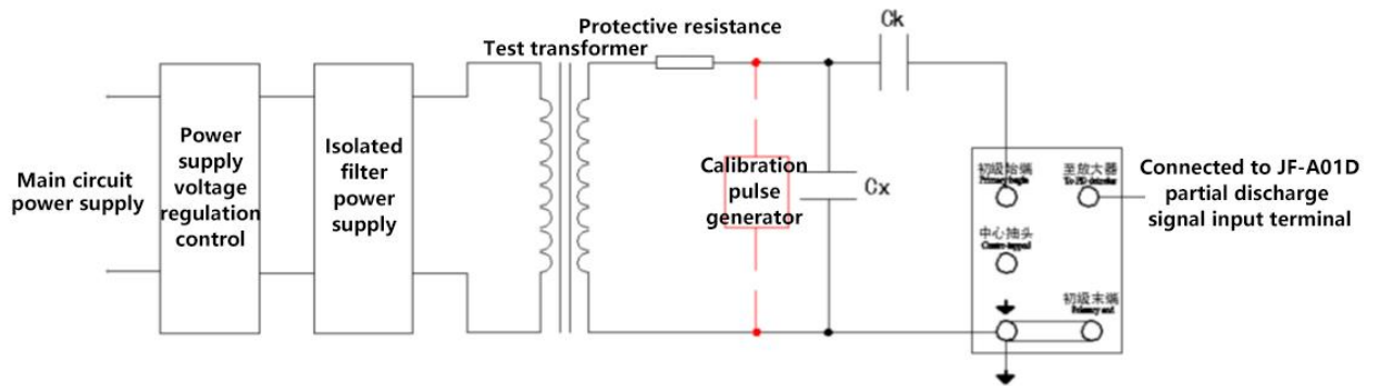
Figure 4 Standard connection circuit of partial discharge test (parallel connection of direct method)
