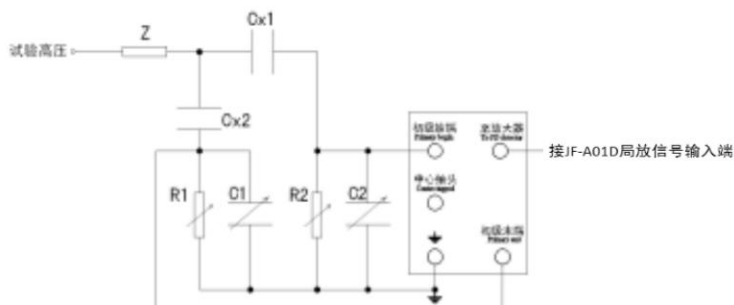
Figure 3d Bridge tapping method
