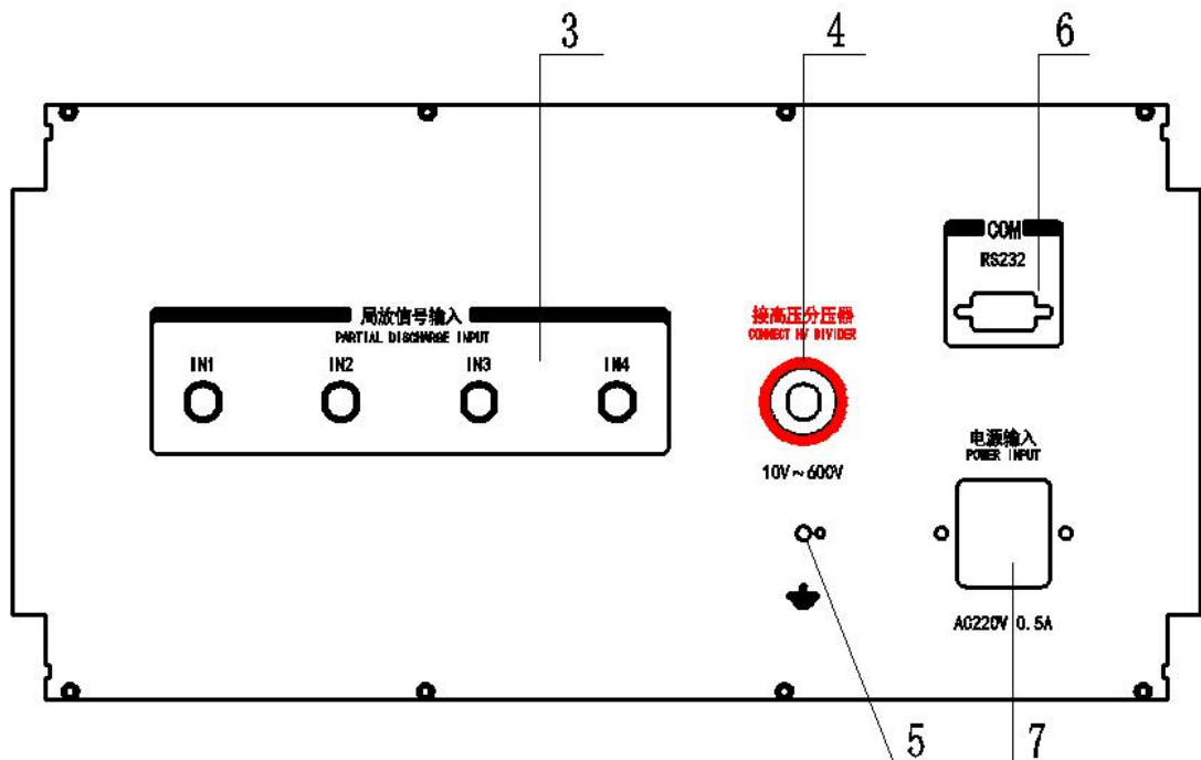
Figure 2b HZJF-9011D Schematic diagram of back panel of partial discharge detector
